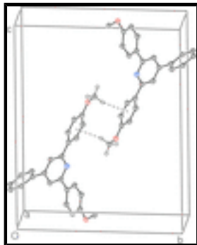
Fig. 2. The one-dimensional chain structure was built by the C—H... \pi H-bond interactions (dashed lines).
