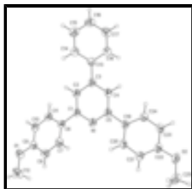
Fig. 1. ORTEP drawing of the title complex with atomic numbering scheme and thermal ellipsoids at 30% probability level.
